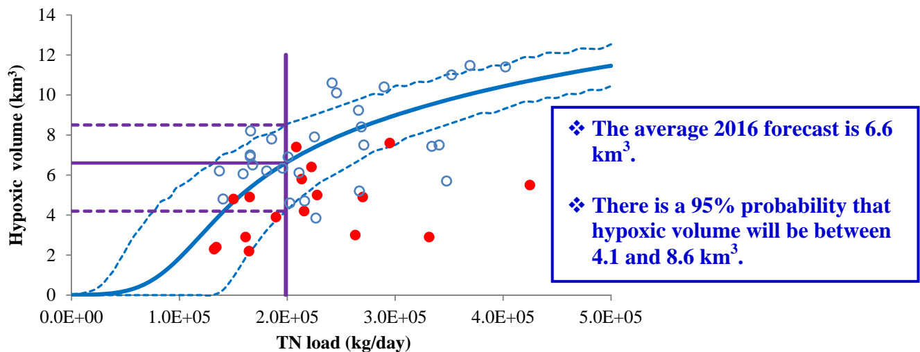
Figure 1. Forecasting relationship of TN vs. Hypoxia volume. The solid blue curve is the response curve (mean value); dashed blue curves are response curve confidence intervals (2.5 and 97.5% values), calibrated to the open blue dots. The open blue dots are observed values for 1985-2013 while the closed red dots are observed values before 1985. The vertical purple line represents the 2016 Jan-May TN load of 197,368 kg/day and the horizontal lines show the forecast hypoxic volume (mean and confidence intervals) associated with this load.
