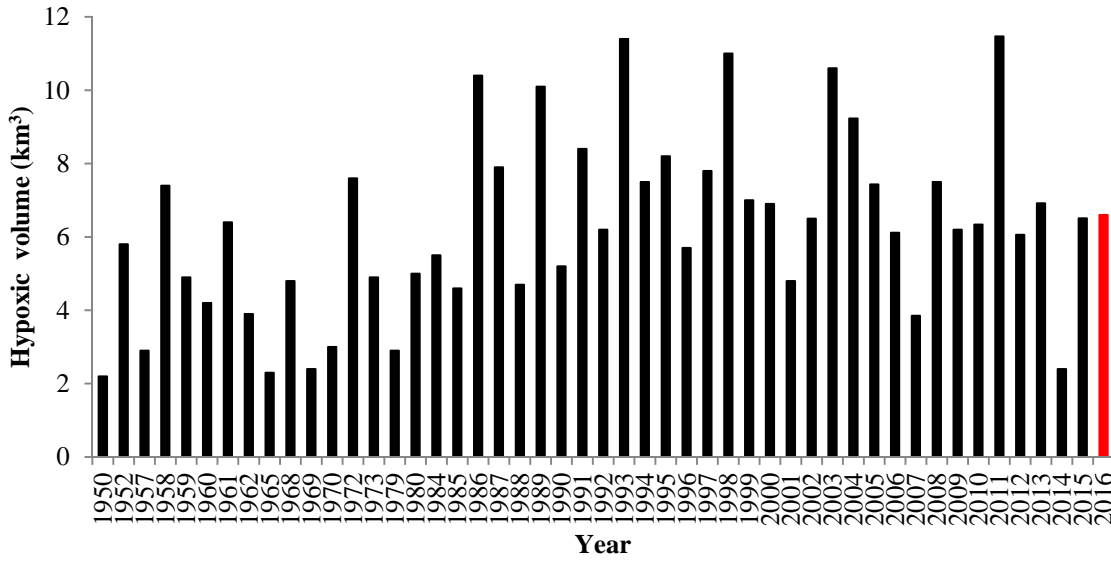
Figure 4. The observed hypoxic volume (km 3 ) for the period of record, the predicted volume in 2016 is in red.
