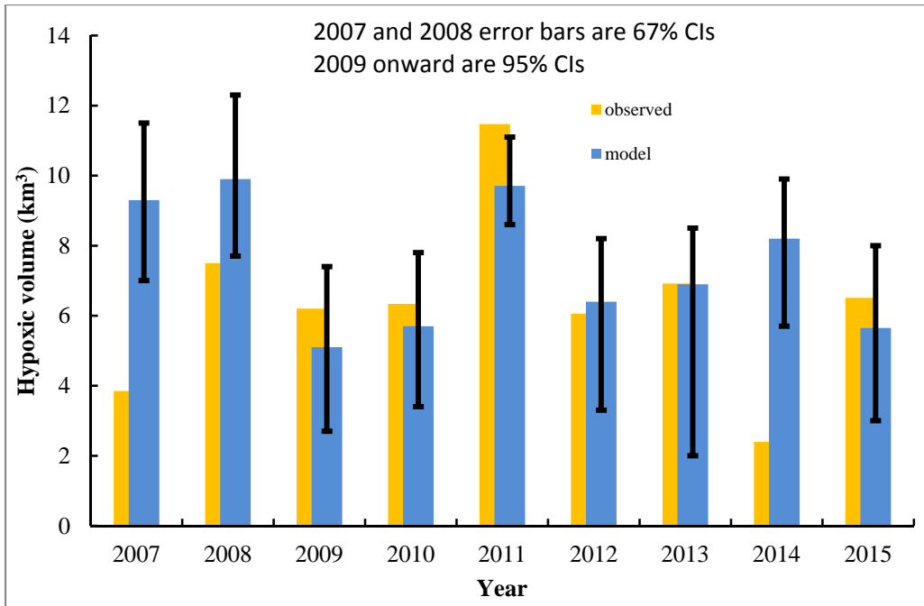
Figure 2. Model forecast and observed hypoxic volume for the years when spring forecasts have been performed. The model calibration has varied over the years. The years 2007 and 2008 used the original model calibration, 2009 used a recalibration with updated load and hypoxic volume information, in 2010-2014 a three year moving window calibration was used (Evans and Scavia 2011), while since 2015 the years 1985-2013 have been used to calibrate the model.
