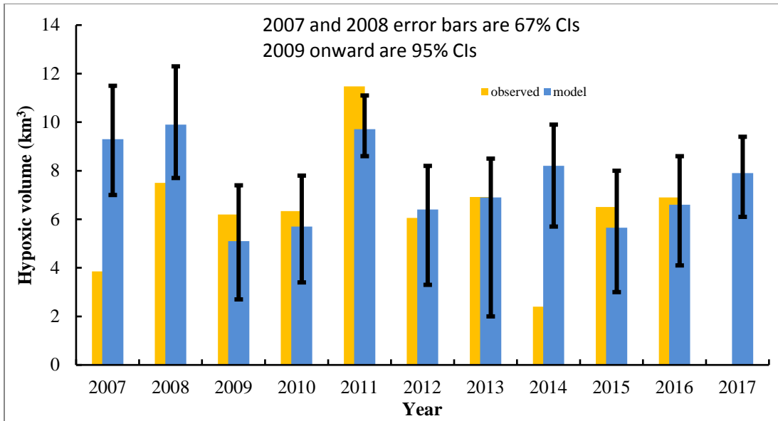
Figure 2. Model forecast and observed hypoxic volume for the years when spring forecasts have been performed. The model calibration has varied over the years. The years 2007 and 2008 used the original model calibration, 2009 used a recalibration with updated load and hypoxic volume information, in 2010-2014 a three year moving window calibration was used (Evans and Scavia 2011), while since 2015 the years 1985-2013 have been used to calibrate the model.
