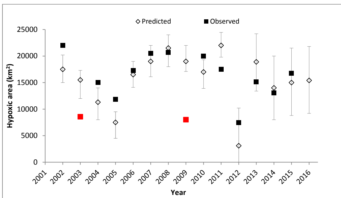
Figure 2: Forecast track record showing model forecast and observed hypoxic area for each year since 2002. “Wind” and “Storm” year observations are indicated in red. Model calibration procedures have varied through time as more has been learned about the drivers of hypoxia in the Gulf. There were no observed hypoxia estimate in 2016.
