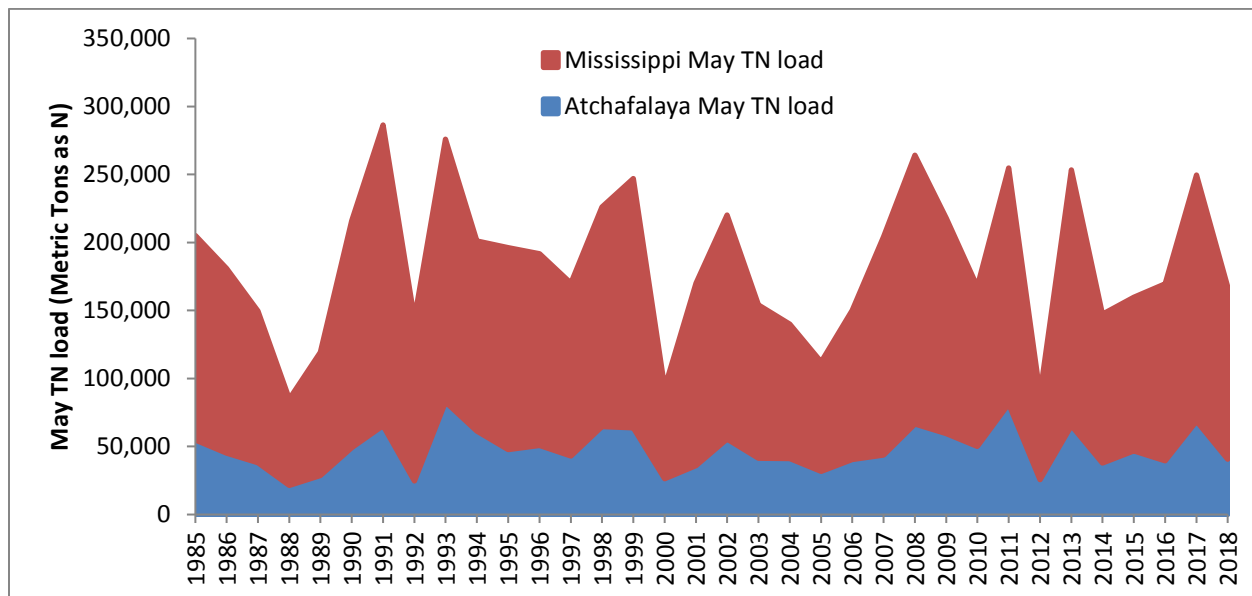
Figure 3: May total nitrogen loads from the Mississippi and Atchafalaya Rivers since 1985. The Mississippi load is the red area and the Atchafalaya load is the blue area such that the height of the combined shaded areas is the total load.
