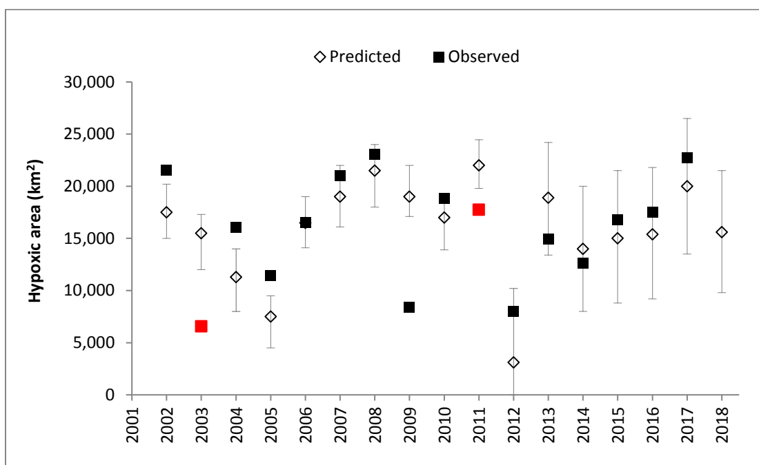
Figure 2: Forecast track record showing model forecast and observed hypoxic area for each year since 2002. “Wind” and “Storm” year observations are indicated in red. Model calibration procedures have varied through time as more has been learned about the drivers of hypoxia in the Gulf.
