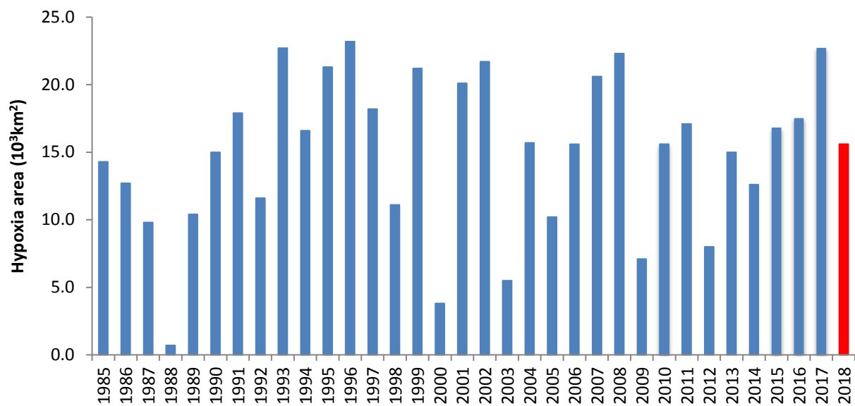
Figure 1: Mid-summer hypoxic area (Obenour et al. 2013 and Rabalais and Turner, LUMCON, 2018). The 2016 value is the average of two 3D ecological model reanalysis project from A. Lewitus, NOAA. 2018 forecast in red.
