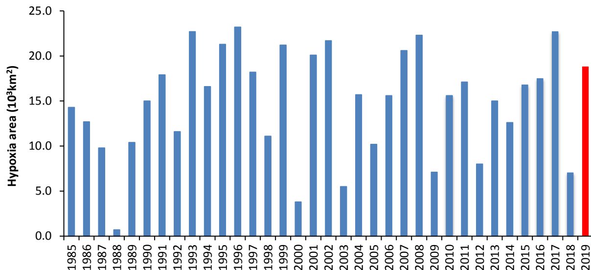
Figure 1: Mid-summer hypoxic area (Obenour et al. 2013 and Rabalais and Turner, LUMCON, 2019). The 2016 value is the average of two 3D ecological model reanalysis project from A. Lewitus, NOAA. 2019 forecast in red.
