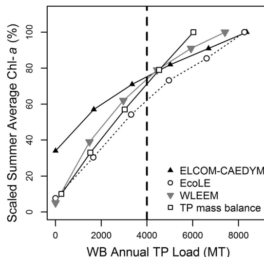
Fig. 3. Average summer chlorophyll- a concentration in the WB predicted by different models as a function of annual WB TP loads. Each response curve has been scaled to 100% at its maximum chlorophyll value to facilitate comparisons. The dashed line represents a 40% reduction from the 2008 WB annual load.
