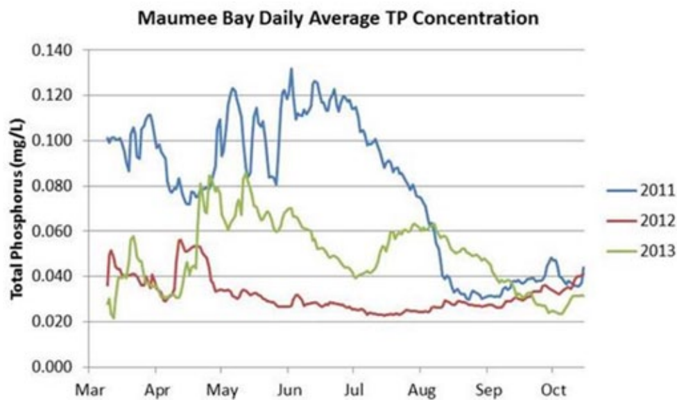
Figure 21. Maumee Bay daily average TP concentration simulated by WLEEM for 2011, 2012, 2013.
