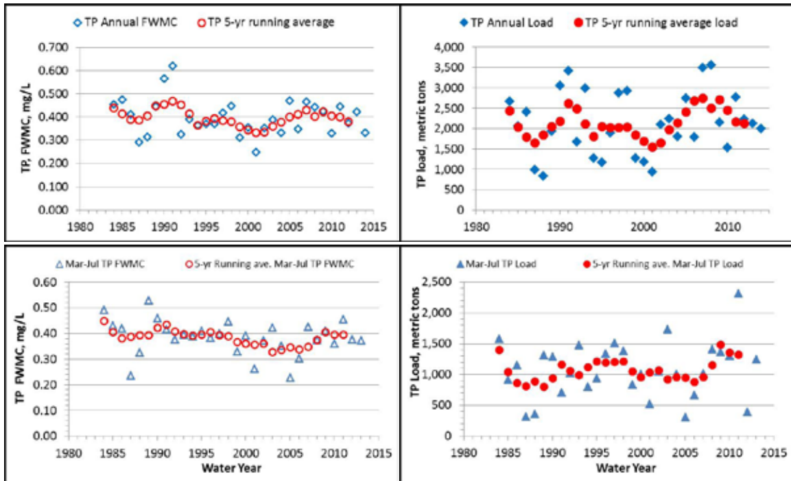
Figure 10. Maume River flow-weighted mean total phosphorus concentrations (left panels) and loads (right panels). Top panels depict annual (water year) values, bottom panels depict March-July "critical period" values. Blue symbols = raw values, red symbols = five-year running averages.
