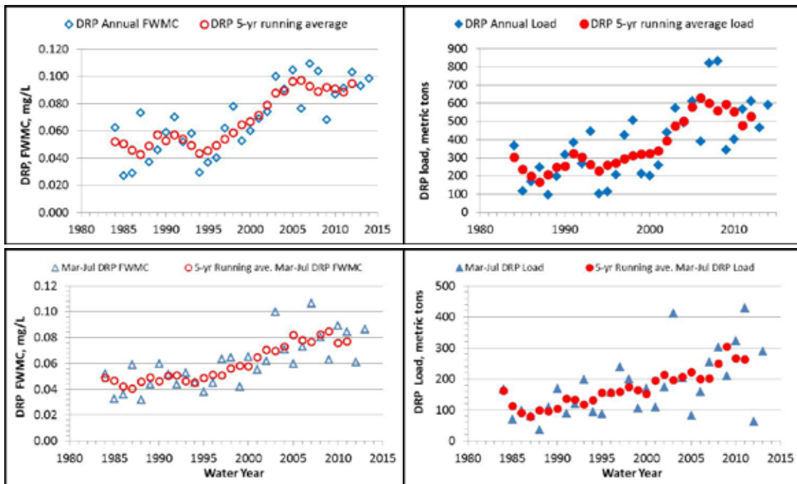
Figure 11. Maume River flow-weighted mean dissolved reactive phosphorus concentrations (left panels) and loads (right panels). Top panels depict annual (water year) values, bottom panels depict March-July "critical period" values. Blue symbols = raw values, red symbols = five-year running averages.
