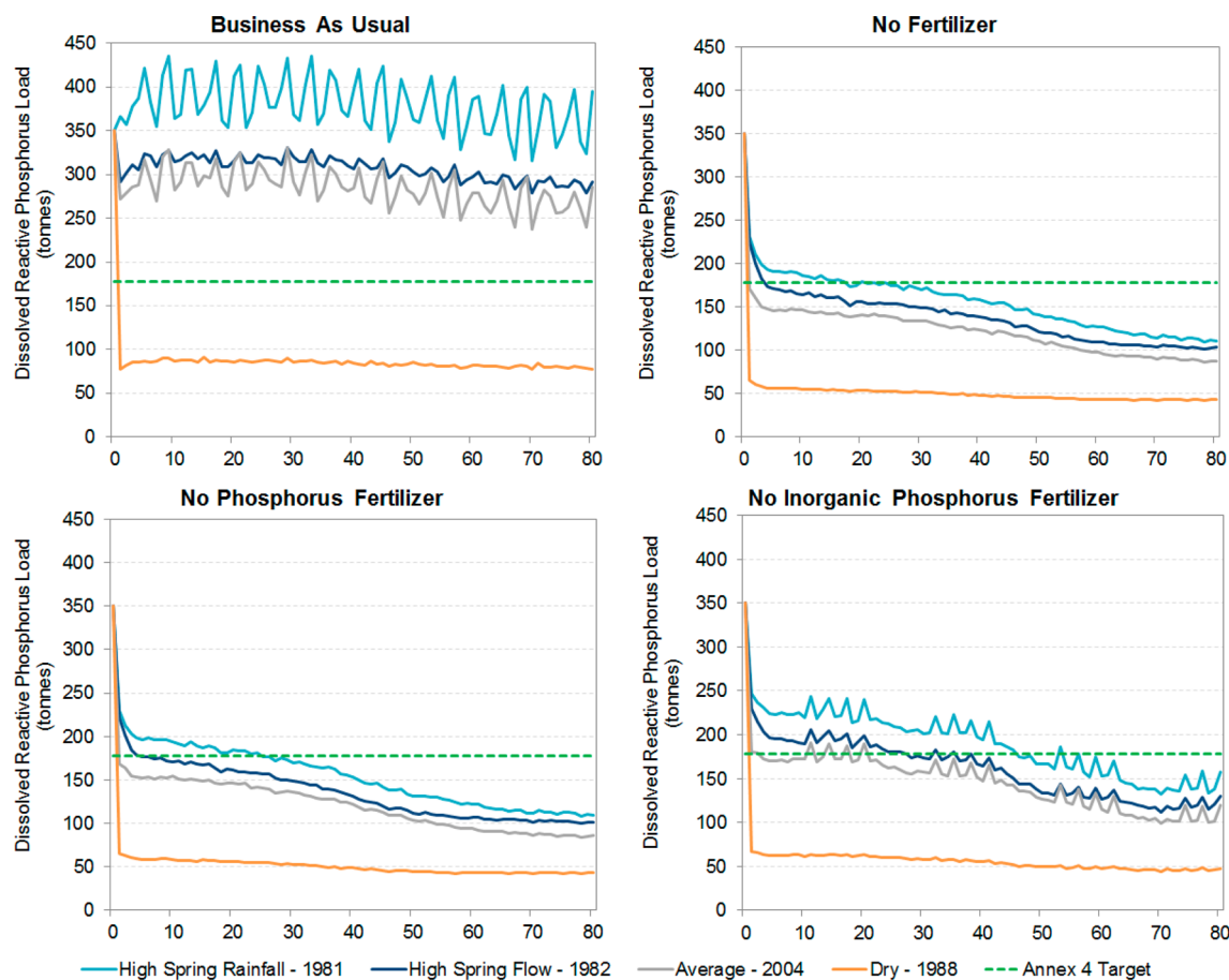
Figure 2. Dissolved reactive phosphorus loads (March to July) under each fertilizer-application-cessation scenario for each type of climate condition across 80 years of simulation. The light-blue line represents high-spring-rainfall conditions (1981), the dark-blue line represents high-spring-streamflow conditions (1982), the gray line represents average climate conditions (2004), the orange line represents dry climate conditions (1988), and the dashed green line represents the GLWQA targets area-weighted to the Heidelberg water-quality station near Waterville, Ohio.
